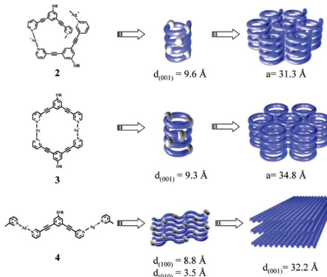
Figure 4. Schematic representation of the self-assembly of 2–4 and their subsequent self-organization.
