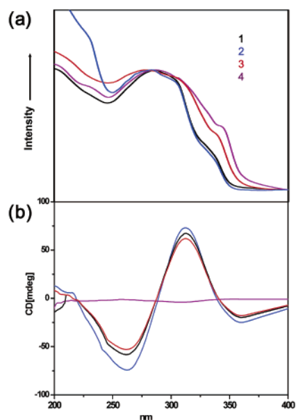
Figure 5. (a) UV spectra of 1–4 in solid state. The spectra have been normalized with respect to their maximum intensity. (b) CD spectra of 1–4 at 25 °C (10 wt % in MeOH).
