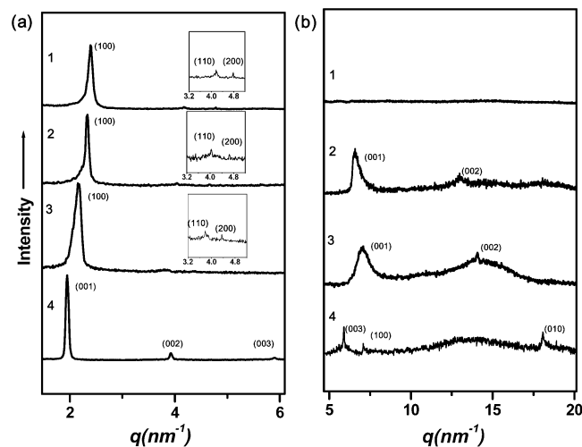
Figure 1. Small-angle X-ray diffraction patterns (a) and wide-angle X-ray diffraction patterns (b) of 1–4 .
