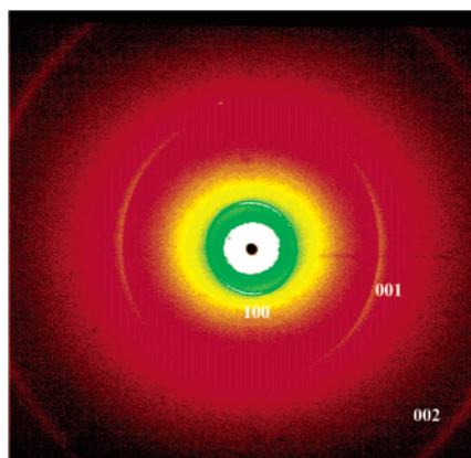
Figure 2. 2-D X-ray diffraction pattern of 3 .
