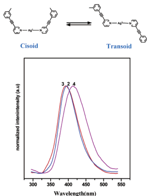
Figure 7. Fluorescence spectra of 2–4 in the solid state.
